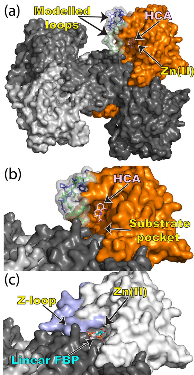
Figure 4. Rearrangement of the substrate pocket caused by HCA binding. (a) Surface rendering of the MtFBA–HCA complex as its tetrameric biological assembly with one MtFBA protomer colored orange, the rest colored various shades of gray, and HCA rendered as pink sticks. Loops that were modeled in due to a lack of electron density are shown as transparent surfaces and either green sticks (residues 167–177) or blue sticks (residues 210–223). (b) Close-up of the substrate binding pocket of the MtFBA–HCA complex. (c) Close-up of the substrate binding pocket for MtFBA (white) bound with linear fructose 1,6-bisphosphate (cyan sticks; PDB entry 3ELF), in which residues 210–223 are colored light blue. In all cases, the zinc ions are rendered as a black sphere.
