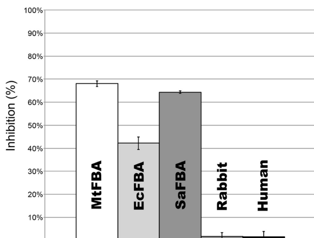
Figure 6. Effectiveness of HCA against class I FBAs and other class II FBAs. HCA at 25 \mu M was tested for its ability to inhibit class II FBAs from E. coli and MRSA as well as class I FBAs isolated from either rabbit or human muscle. Error bars represent the standard deviations from the average.
