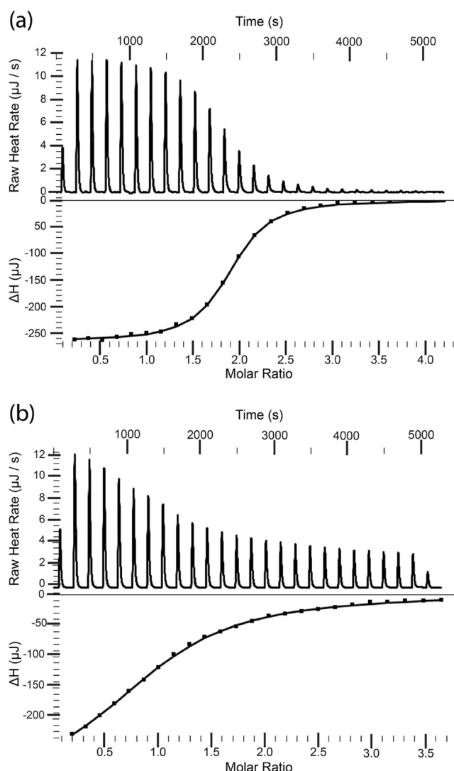
Figure 2. ITC binding of MtFBA with HCA. The top panel represents the raw heat data from 25 injections at 25 ^{\circ}\text{C} , and the bottom panel shows the integrated heat peak areas plotted vs the molar ratio of (a) HCA to \text{ZnCl}_2 or (b) HCA in the presence of excess \text{ZnCl}_2 to MtFBA. The last five data points were averaged for the heat of dilution and subtracted from the rest of the data. The lines represent the best fits to an independent mode. This figure was generated using the NanoAnalyze software provided by TA Instruments.
