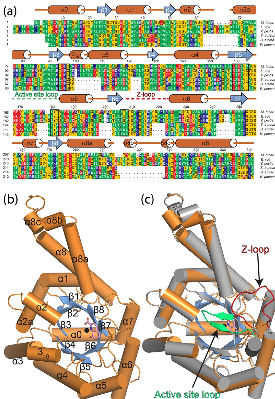
Figure 3. Sequence alignment of class II FBAs and X-ray structure of MtFBA in complex with HCA. (a) FBAs are from M. tuberculosis (M. tuber; NP_334786), E. coli (E. coli; PDB entry 1B57_A), Yersinia pestis (Y. pestis; ZP_04518851), S. aureus (S. aureus; Q5HE75), Bacillus anthracis (B. anthrac; PDB entry 3Q94_A), and Klebsiella pneumoniae (K. pneum; ZP_14594173). The secondary structure of the MtFBA-HCA complex according to Defined Secondary Structure of Proteins (DSSP) is shown as orange cylinders (helical regions), blue arrows (β-sheets), and orange lines (loops). Dashed lines represent residues for which electron density was not defined in the crystal structure. Breaks denote regions where MtFBA does not have residues. Black brackets indicate residues that are part of MtFBA's active site. (b) Cartoon rendering of the MtFBA-HCA protomer. Helical regions are represented as cylinders and β-strands as arrows. Helices and loops are colored orange and β-strands blue; HCA is shown as pink sticks, and zinc ion is shown as a black sphere. (c) Same MtFBA-HCA complex shown in panel b but overlaid with the MtFBA-PGH complex (PDB entry 4DEL) colored gray. Residues 167–177 (green) and 210–223 (red) for which density is observed in the MtFBA-PGH structure but not in the MtFBA-HCA structure.
