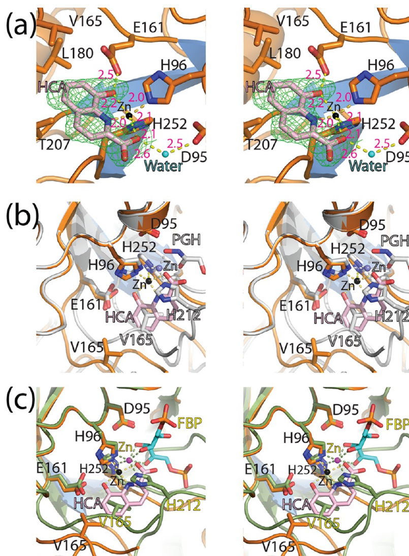
Figure 5. Comparison of the active sites of class II FBAs. (a) Wall-eyed stereoview close-up of HCA interacting with MtFBA and zinc. Green mesh represents F_o - F_c density scaled to 3\sigma ; black labels indicate MtFBA residues, and hot pink labels and dashed lines indicate distances measured in angstroms. (b) Wall-eyed stereoview of MtFBA (orange) bound to HCA (pink) interacting with Zn (black) overlaid with MtFBA interacting with PGH (gray; PDB entry 4DEL) and Zn (purple), with dashed lines indicating bonding interactions. (c) Wall-eyed stereoview of MtFBA bound to HCA interacting with Zn colored as in panel b overlaid with MtFBA (green) interacting with FBP (cyan; PDB entry 3ELF) and Zn (magenta) with dashed lines indicating bonding interactions.
